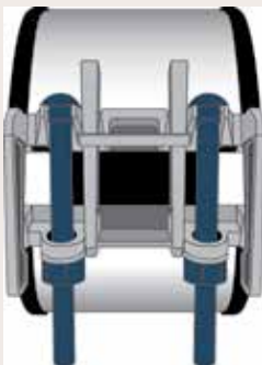
Body 100% Insulated from Ductile Iron Pipe with Gasket and Insulating Boot to Prevent Bi-Metallic Corrosion
